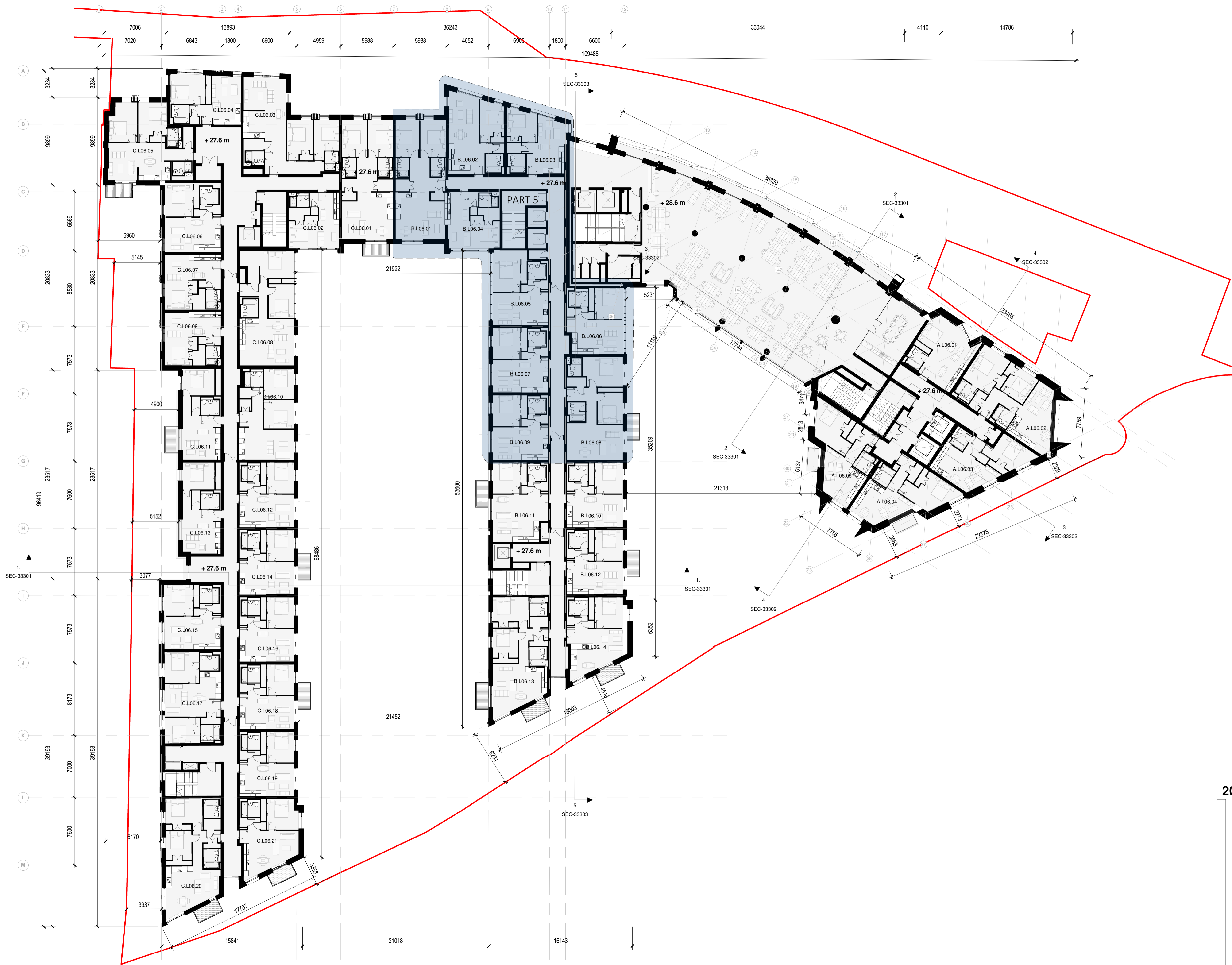
Proposed 6th Floor Plan 1:200
